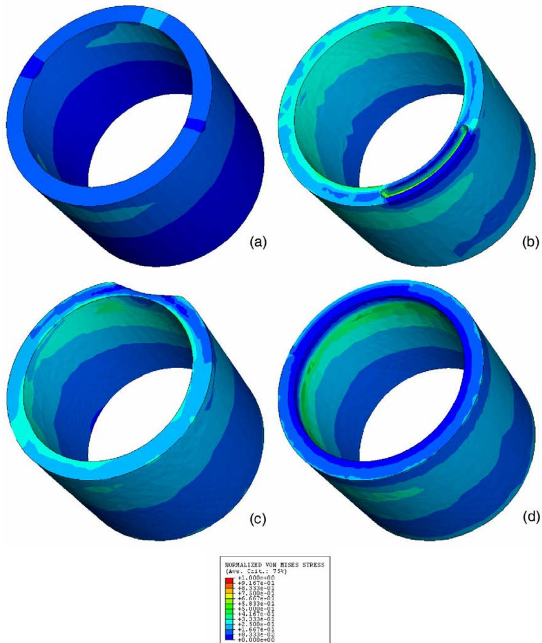
Figure 9. Normalized von Mises stress distribution in the cement layer computed with the finite element method in the case of: (a) cement layer without defects; (b) gas bubble included within the cement layer; (c) detachment at the dentin/cement interface; (d) traces of primary cement included within the secondary cement.
