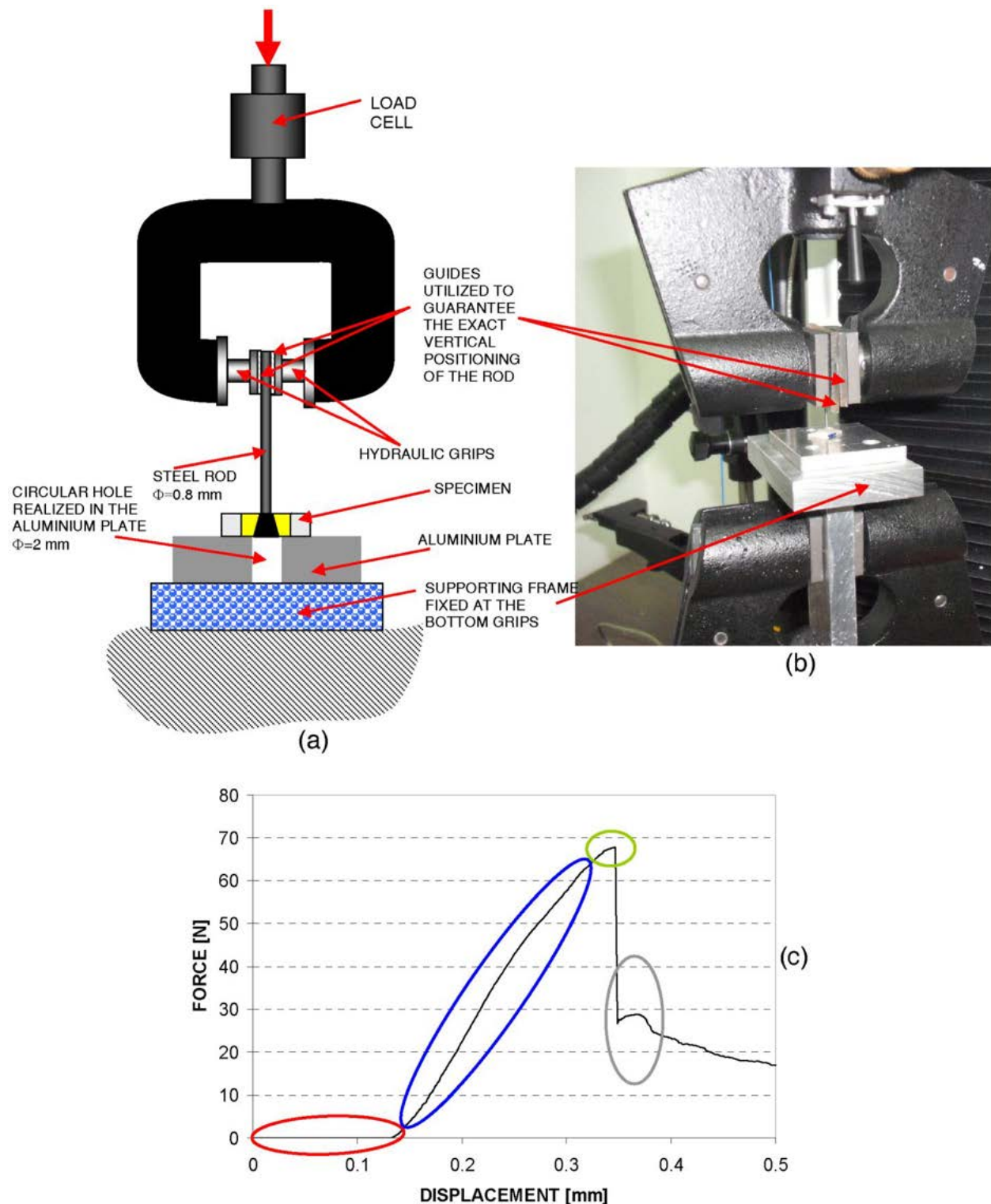
Figure 2. Schematic (a) and picture (b) of the loading system utilized to perform the micro-push-out test; (c) typical force-displacement curve registered for the generic sample submitted to micro-push-out test. Four different regions can be distinguished. An initial region (highlighted in red) in which, due to the clearance existing between the sample and the aluminium plate, as well as the rod tip and the sample, small values of force are registered against large displacement values; a second region (highlighted in blue) where a quasi-linear increase of the force with the displacement occurs; a third region (highlighted in green) where a sudden decrease of the force occurs, which indicates that the critical condition of failure has been reached; a fourth region (highlighted in grey) where, due to the fact that the portions of the bonding area at the post-cement interface that did not fail yet oppose the further displacement of the rod, a small increase of the force is observed.
